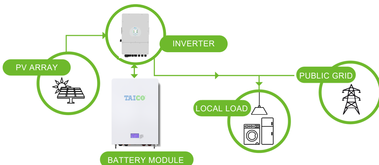
Application Schematic
